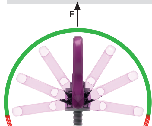
Pic. 10: Pivoting area (green = permitted loading direction)
