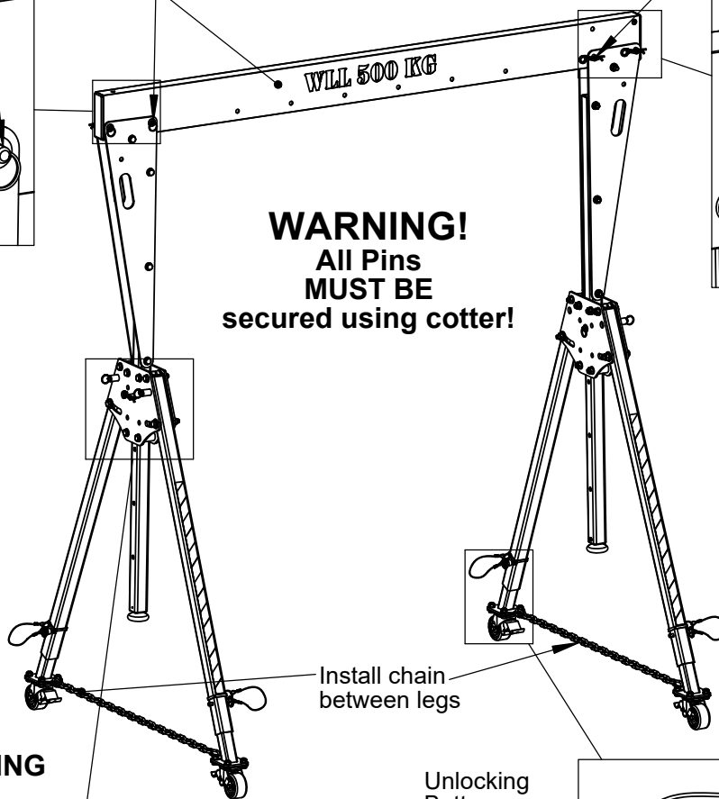
Pin with cotter
